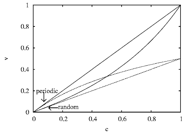
FIG. 2. Velocity of the walker in the original (solid) and in the modified (dashed) burnt-bridge model, for random and periodic bridge distributions.
